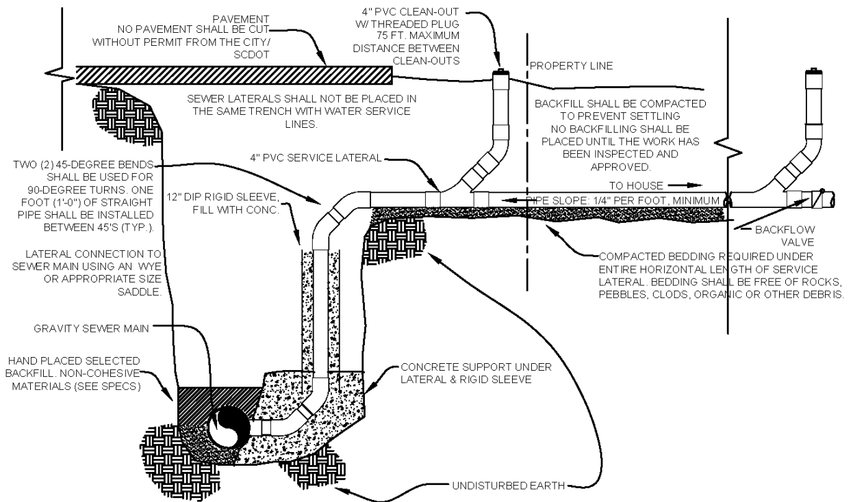
TYPICAL DETAILS OF VERTICAL RISER
