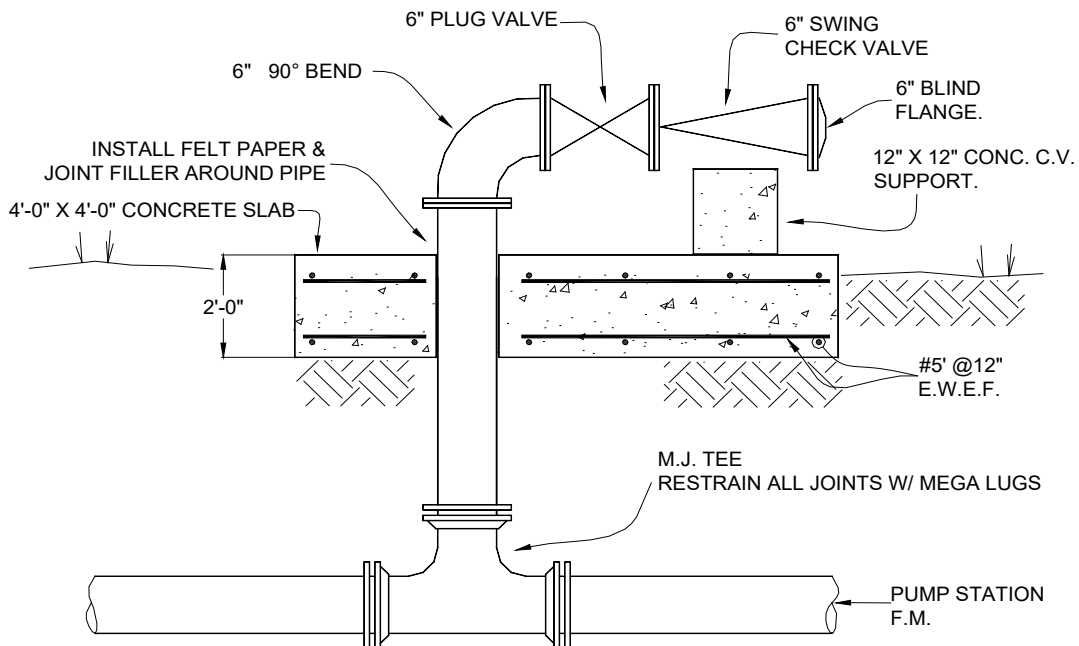
SD-17, EMERGENCY PUMP STATION BY-PASS CONNECTION, N.T.S
