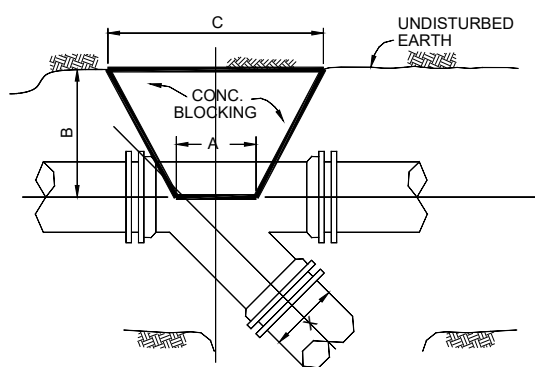
WYES
