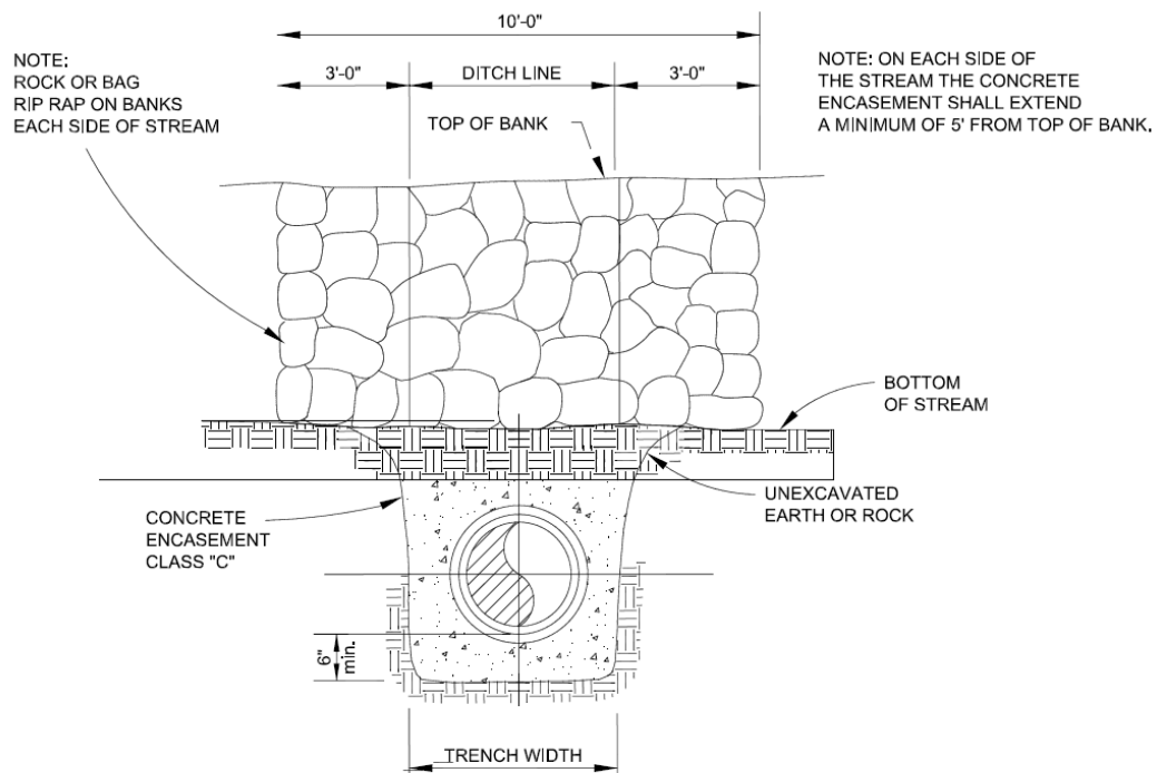
TYPICAL STREAM CROSSING DETAIL
