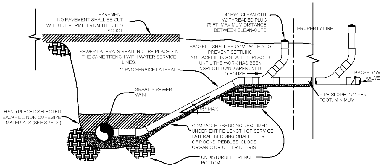
TYPICAL DETAILS OF SANITARY HOUSE SERVICE LINE
