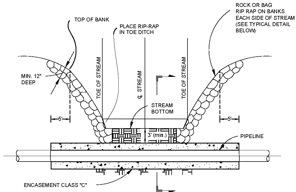
TYPICAL DETAIL FOR RIP RAP ON BANKS OF STREAM
