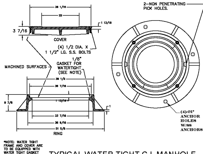
TYPICAL WATER TIGHT C.I. MANHOLE FRAME & COVER (OUTSIDE ROAD RIGHT-OF-WAY) N.T.S.
