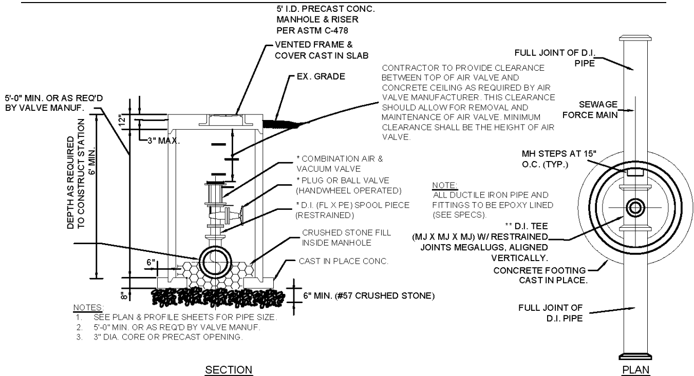
SD-18, SEWER FORCE MAIN AIR RELEASE VALVE INSTALLATION, N.T.S
